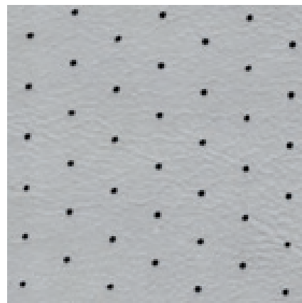
Ford/GM/Chrysler Euro Hole Distance: 16.0mm x 4.61mm Pin Size: 1.4mm Hole Size: 1.2mm (+/- 0.2mm)
