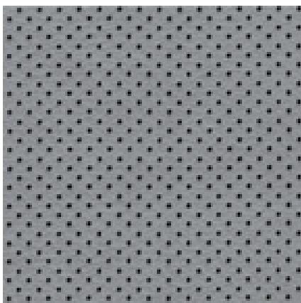
Ford Micro / GM Mini Hole Distance: 3.6mm x 1.8mm Pin Size: 1.1mm Hole Size: 0.9mm (+/- 0.2mm)
