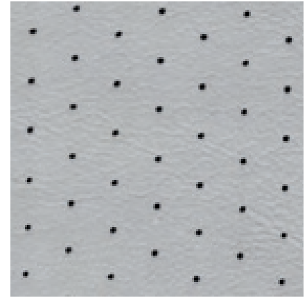
GM/Chrysler Standard Hole Distance: 9.6mm x 4.8mm Pin Size: 1.3mm Hole Size: 1.1mm (+/- 0.2mm)
