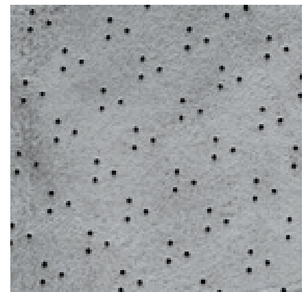
Chrysler Tri-Star Hole Distance: 13.75 mm x 6.5mm Pin Size: 1.1mm Hole Size: 0.9mm (+/- 0.2mm)
