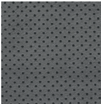
Ford Mini / Chrysler Axis II Hole Distance: 5.0mm x 2.5mm Pin Size: 1.3mm Hole Size: 1.1mm (+/- 0.2mm)
