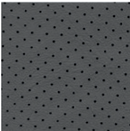
Ford Standard / GM Small Hole Distance: 7.0mm x 3.5mm Pin Size: 1.3mm Hole Size: 1.1mm (+/- 0.2mm)
